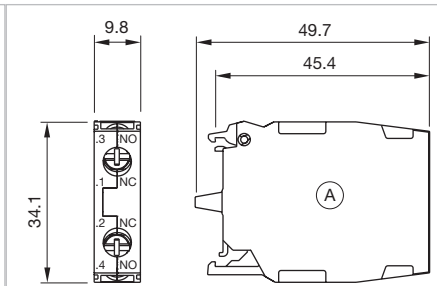
Dimensions [mm] A = Screw terminal for Part No. 45-312.1Z10, 45-312.1X10
