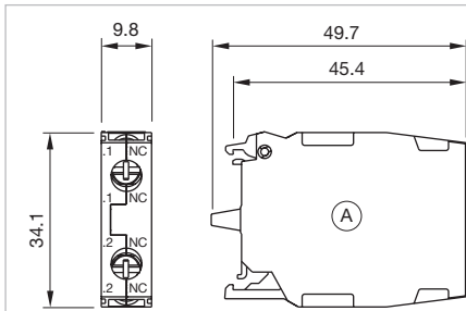
Dimensions [mm] A = Screw terminal for Part No. 45-311.1Z10, 45-311.1X10
