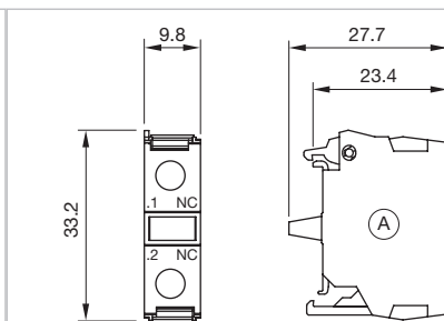
Dimensions [mm] A = Screw terminal for Part No. 45-312.1Z10, 45-312.1X10
