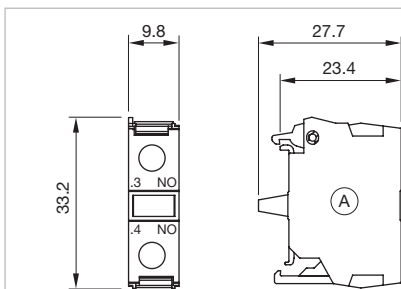
Dimensions [mm] A = Screw terminal for Part No. 45-311.1Z10, 45-311.1X10
