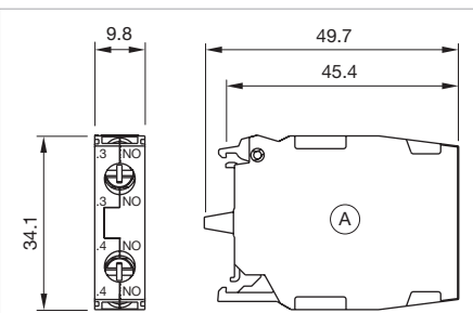
Dimensions [mm] A = Screw terminal for Part No. 45-313.1Z10
